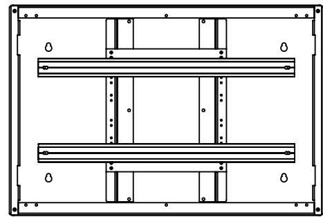
Front View Without Door & Escutcheon
