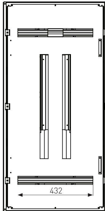
Front View without Door
