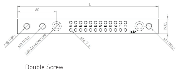
Double Screw
